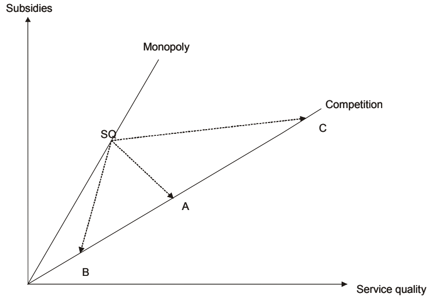
Figure 1: Feasible subsidy/quality-bundles
